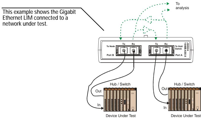
J6832A Gigabit Ethernet LIM in Pass-Thru Connection
